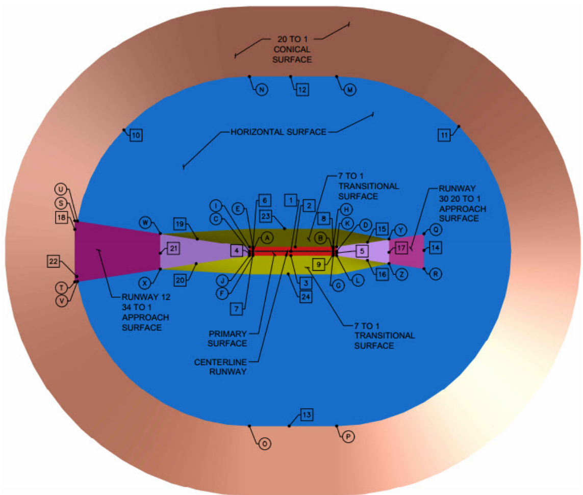
FIGURE 1: PART 77 LINE AND POINT DIAGRAM
