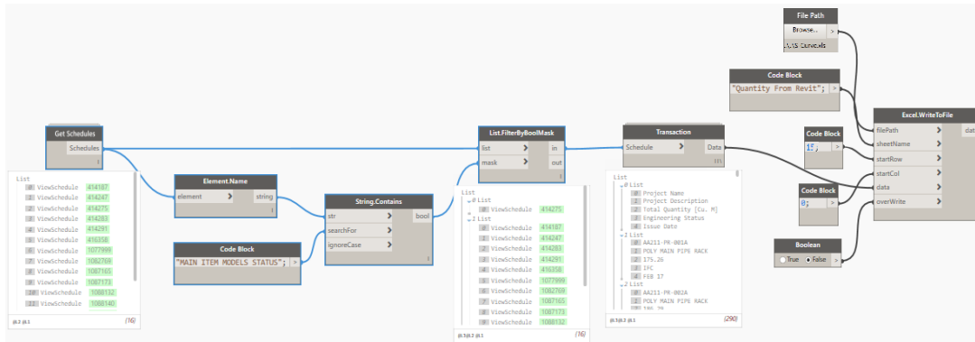
Capture of our Dynamo Script
